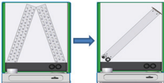
RTPF A-COIL
